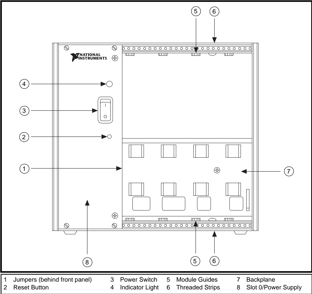
Figure 2-2. SCXI-1000DC Front View Diagram
