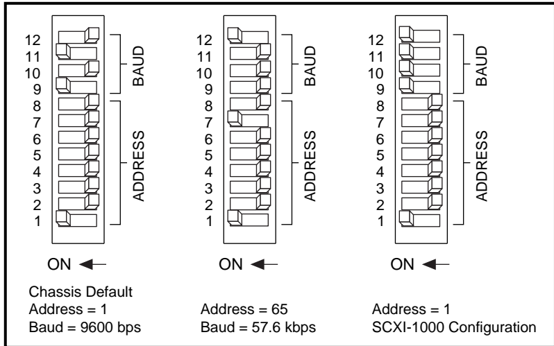
Figure 2-11. Baud Rate and Address Setting Examples
