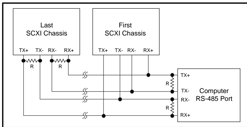
Figure 2-12. RS-485 Connections for Two SCXI-2000 Chassis
