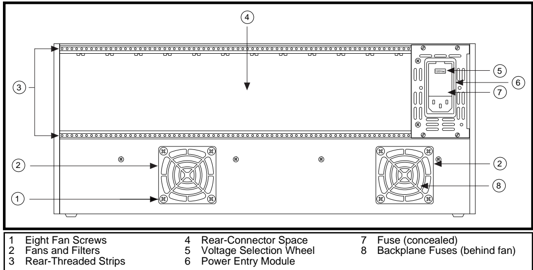
Figure 2-6. SCXI-1001 Rear View Diagram
