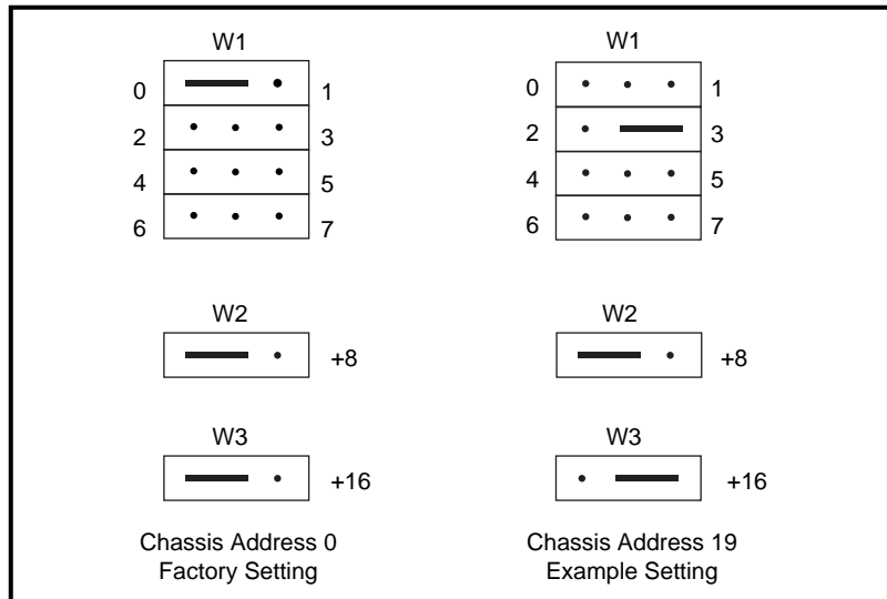
Figure 2-10. SCXI-1000DC Chassis Address Jumper Settings
