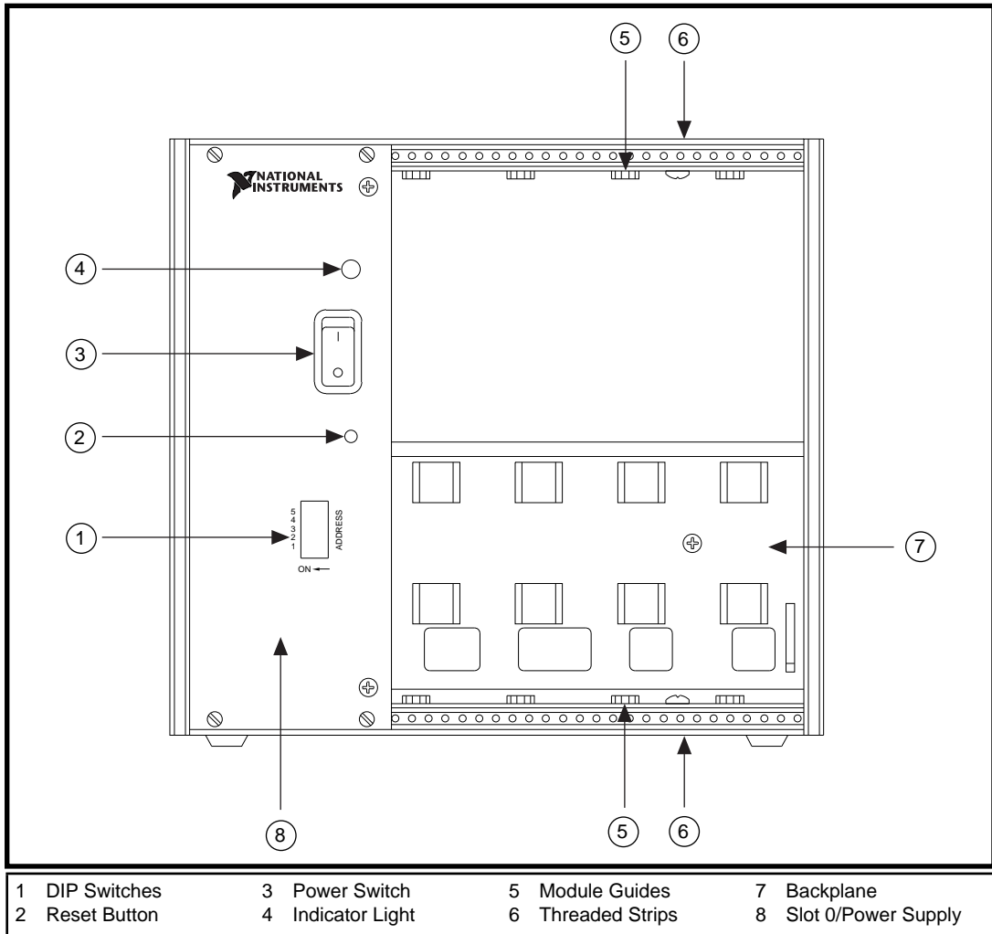
Figure 2-1. SCXI-1000 Front View Diagram
