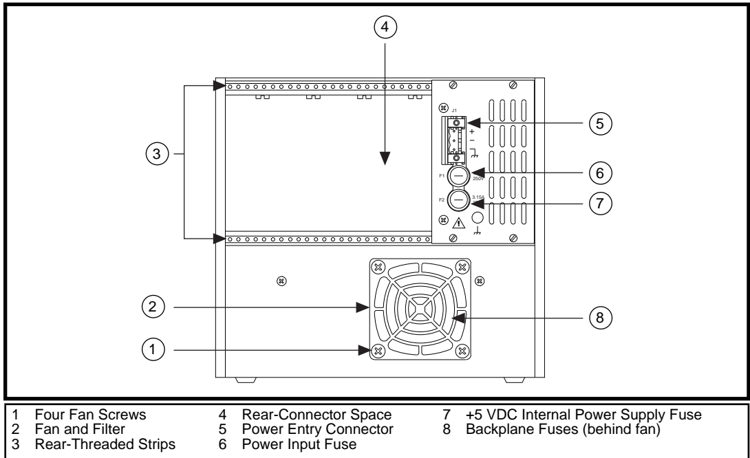
Figure 2-7. SCXI-1000DC Rear View Diagram
