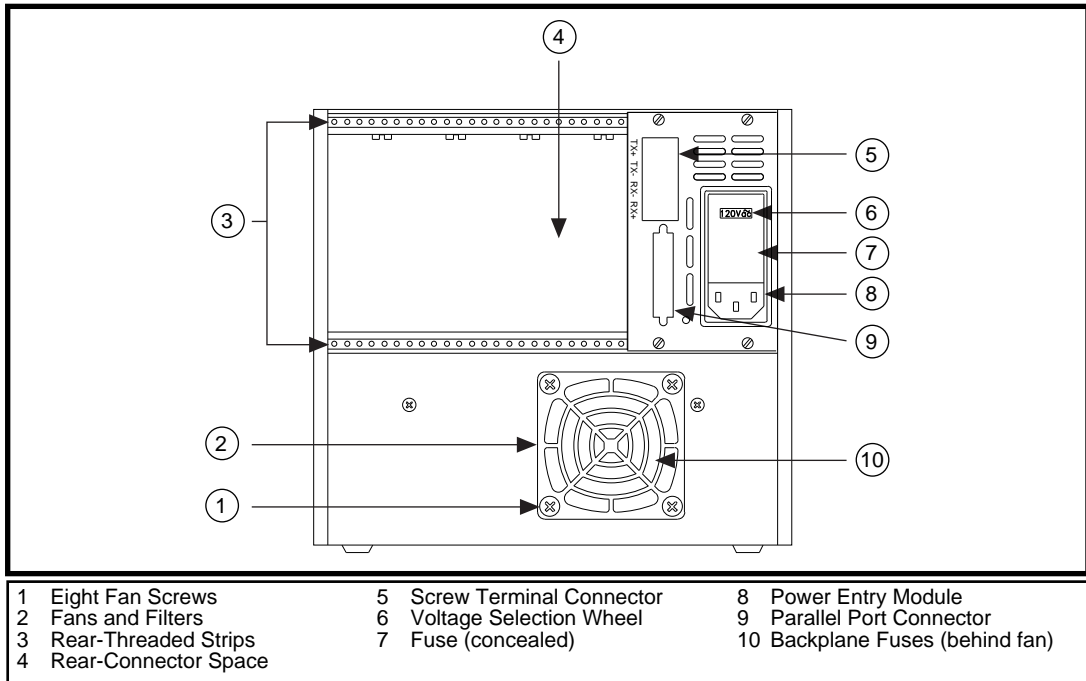
Figure 2-8. SCXI-2000 Rear View Diagram
