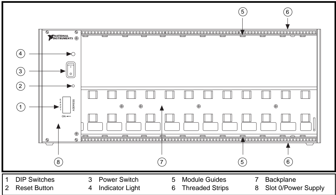
Figure 2-3. SCXI-1001 Front View Diagram
