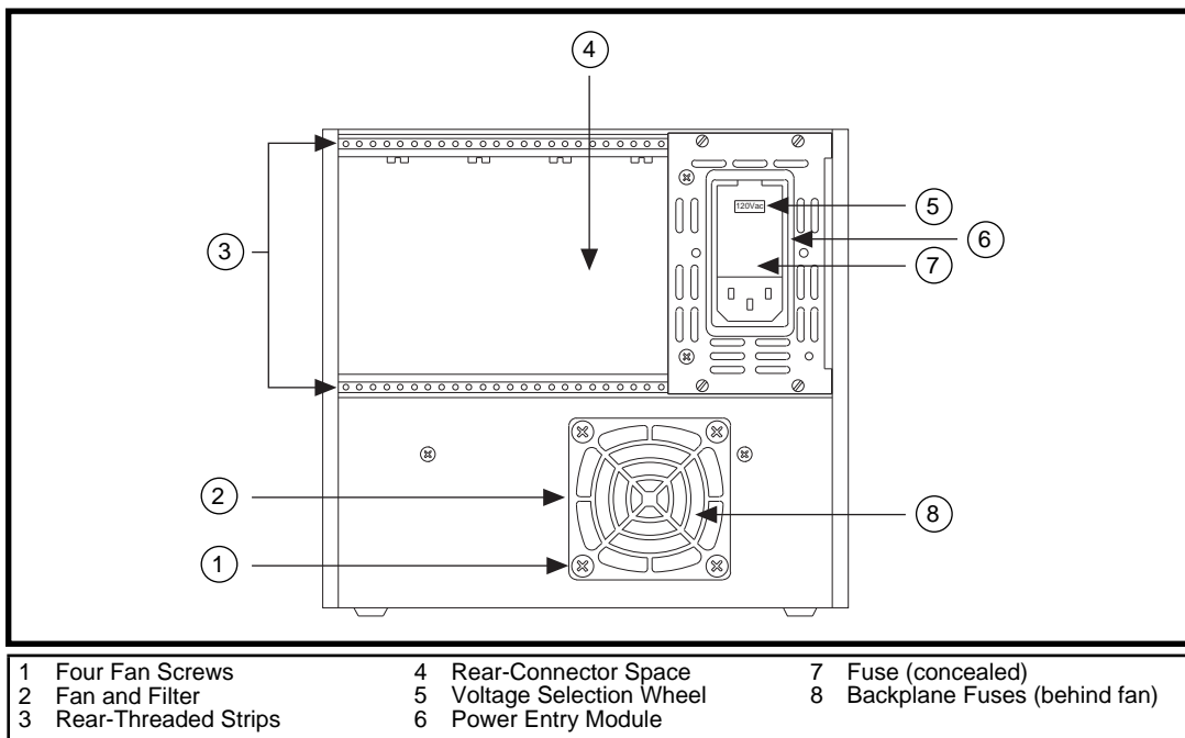
Figure 2-5. SCXI-1000 Rear View Diagram
